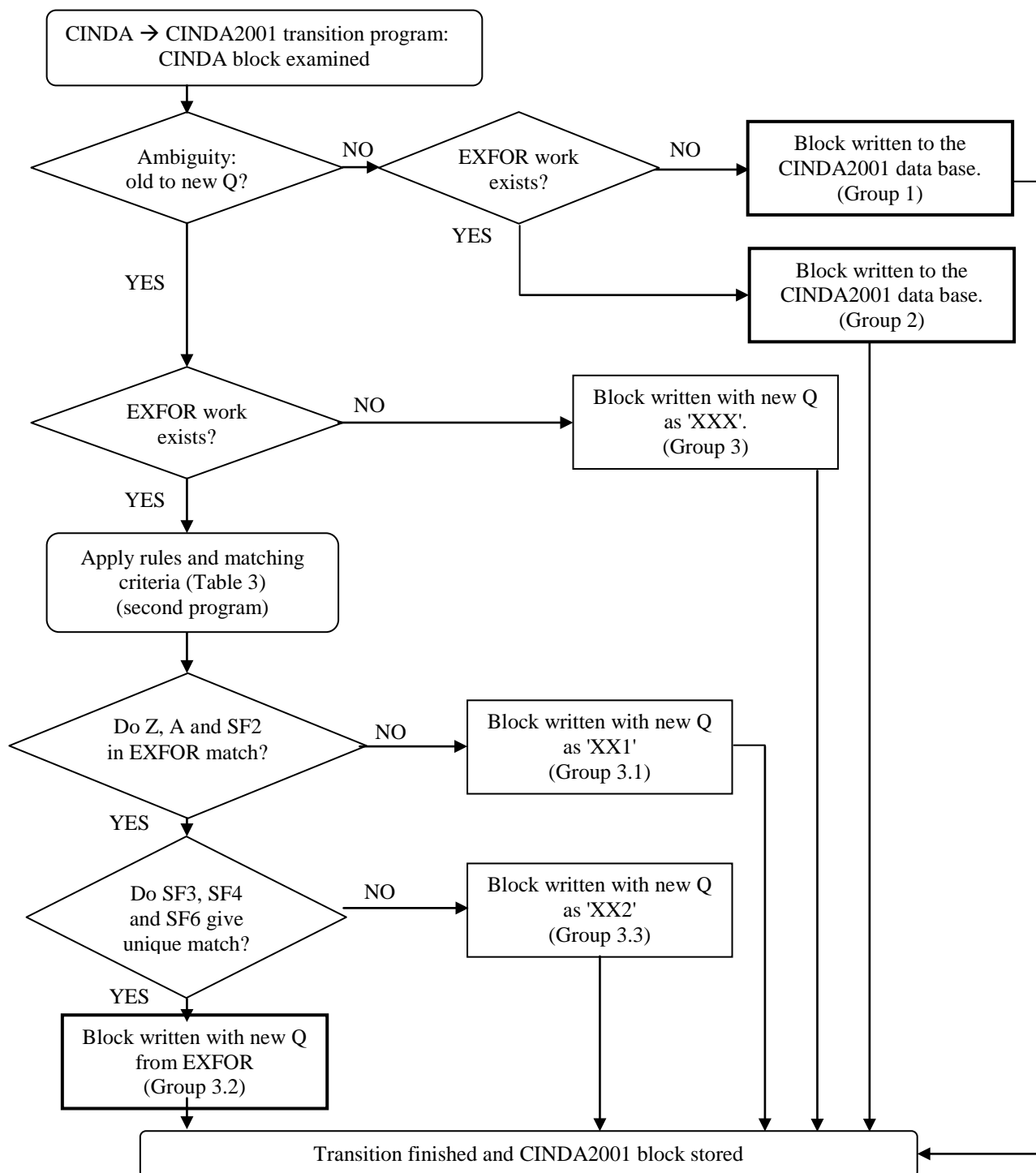
Figure 1. Schematic flow chart of the set of transition programs for the CINDA to CINDA2001 conversion.
